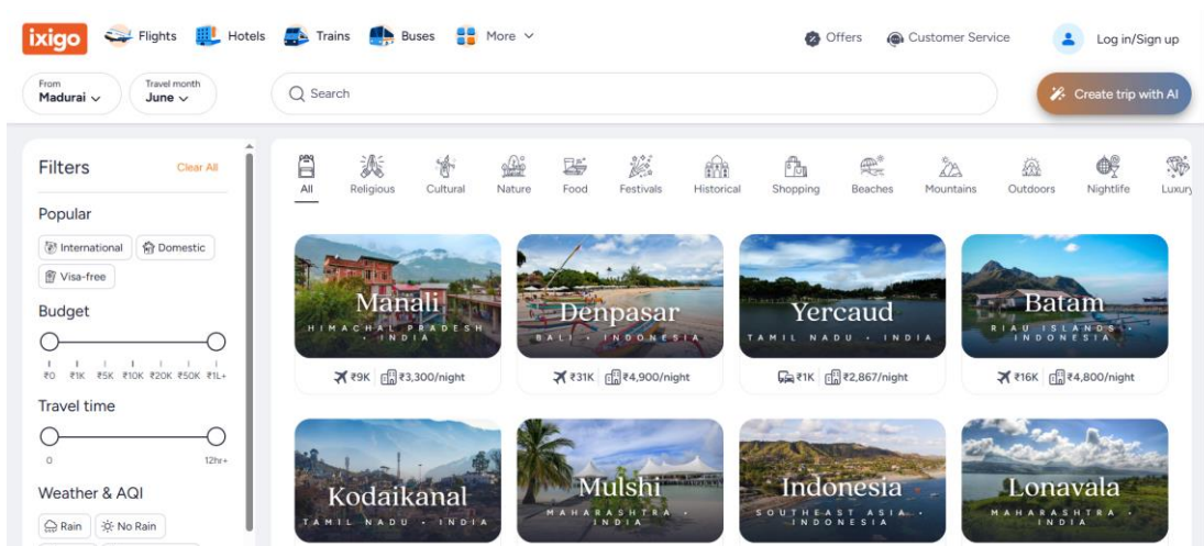
Fig 1: plan_page_navigation
